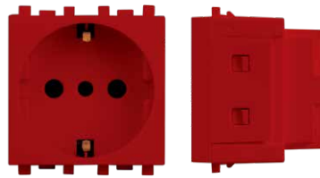
Socket German type description: 16A / (Red) code: CLA 30 297
